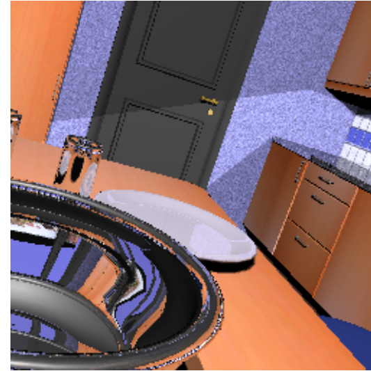
static scene
