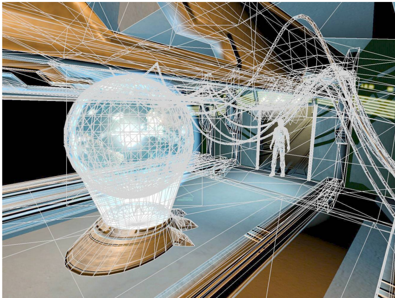
Visible geometry
