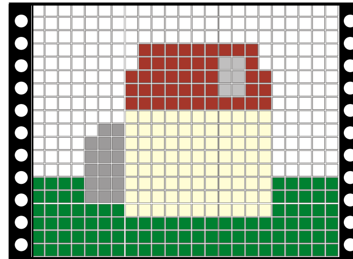
Color Buffer
