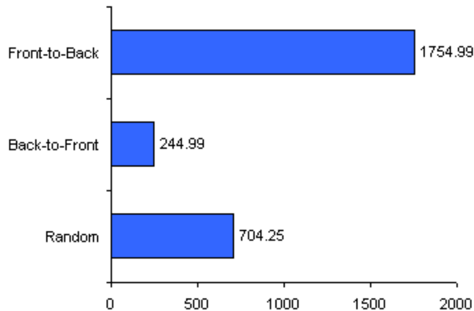
Scene Order Rendering Performance - 8 Layers 1280x1024
