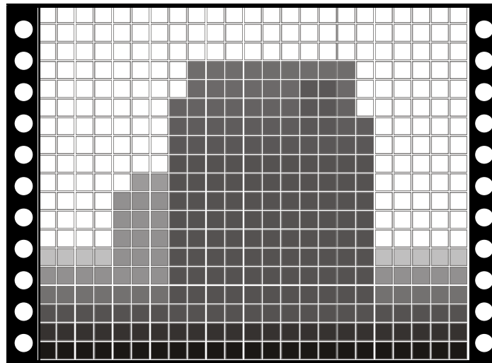
Z-Buffer
