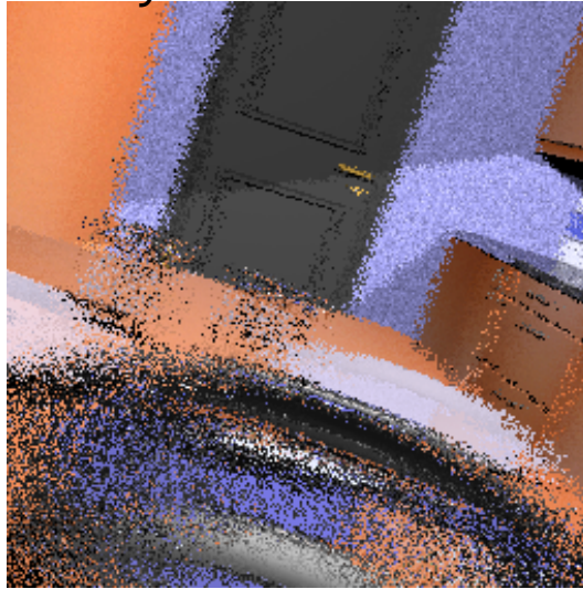
dynamic scene
