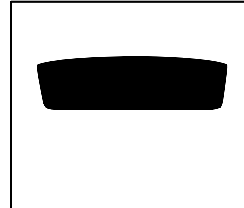
Stencil Buffer
